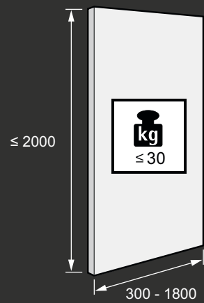
Door size and door weight
