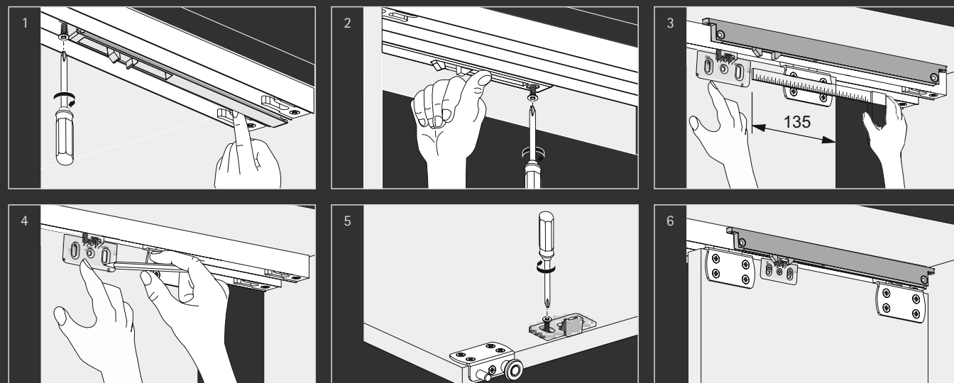
Set contains fitting, profile and silent system
